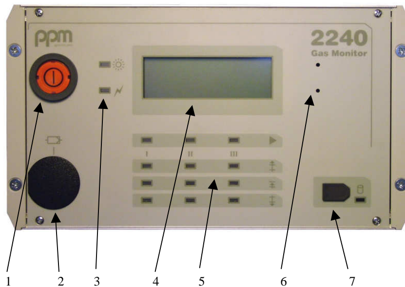
Fig. 1 Front View
